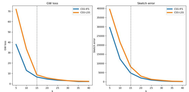
Fig. 10: Corner Flow : Global GW losses and global sketch errors for varying k , the number of basis trees, using IFS and LSS.
