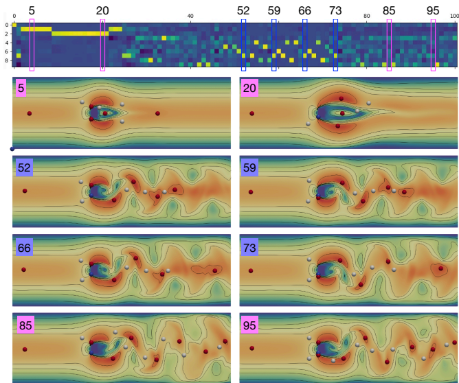
Fig. 13: Sketching the Square Cylinder Flow dataset with IFS. Top shows the coefficient matrix. Bottom shows instances of the scalar fields.
