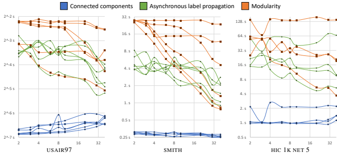
(b) Compute time for small (USAIR97), medium (SMITH), and large (HIC 1K NET 5) graphs across all topological lenses. The plots show time in seconds vertically, and the number of cover elements horizontally. Instability is associated with variability in clustering time.
