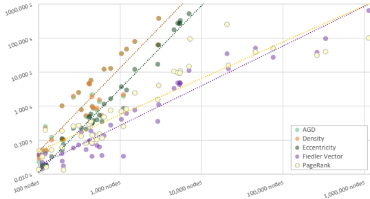
(a) Compute time against the number of nodes for each topological lens. Dotted lines are power regressions. The results show that PageRank (yellow) and Fiedler vector (purple) calculations scale much better than AGD (teal), density (orange), and eccentricity (green).
