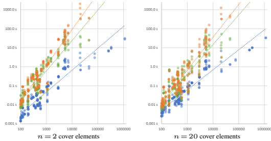
(c) Compute time for all graphs and lens functions for (left) n = 2 and (right) n = 20 cover elements. The plot shows the time in seconds vertically, and the number of input graph nodes ( |V| ) horizontally. The power regressions (dashed lines) show that the size of the input graph and the clustering algorithm have an influence on the compute time.
