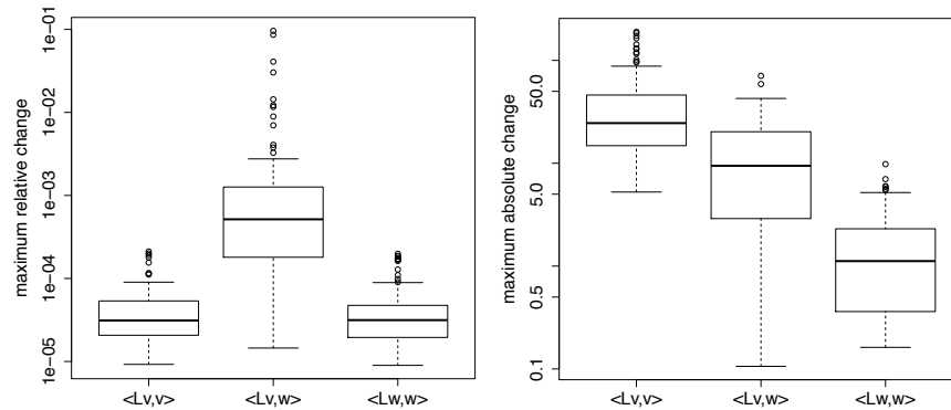
Fig. 4: Maximum amount of change in inner products for each subject. The left plot shows the maximum relative change of each subject x = \langle \cdot, \cdot \rangle is computed by \max_{0 \leq t \leq 1} ((x_t - x_0)/x_0) . The right plot shows the maximum absolute change of each subject, computed as \max_{0 \leq t \leq 1} (x_t - x_0) .
