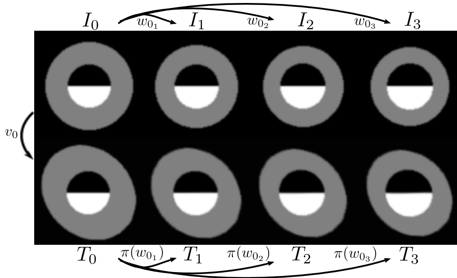
Fig. 1: Results of parallel translating w_{0_n} for each I_0 \dots I_3 to the template space T_0 to produce the transformed images T_1, T_2, T_3 .
