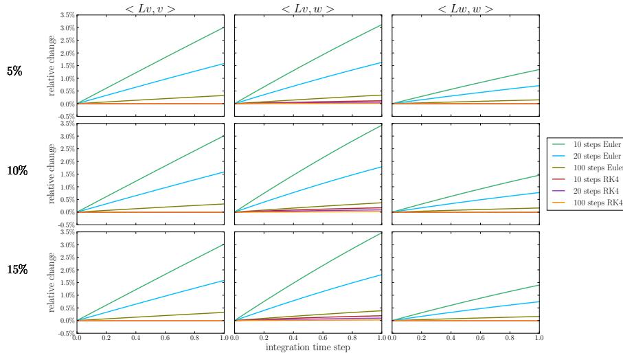
Fig. 2: Percent relative change of the inner product over the integration time from 0 to 1. Where relative percent change of x = \langle \cdot, \cdot \rangle is computed by 100*(x_t - x_0)/x_0 for each time step t . The rows correspond to results for 5%, 10% and 15% simulated atrophy respectively.
