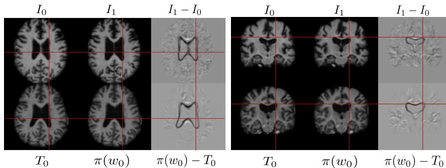
Fig. 3: Axial and coronal views of the results of parallel translating w_0 along v_0 to the template space T_0 to produce the transformed image \pi(w_0) . The top row in each group consists of the original images from a subject with Alzheimer’s, I_0 and I_1 as well as the difference image I_1 - I_0 . The bottom row in each group consists of the original template image from a control subject T_0 , the parallel translated image \pi(w_0) , and the difference image \pi(w_0) - T_0 .
